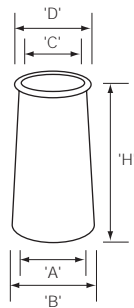
Round to Tapered Type 5E
