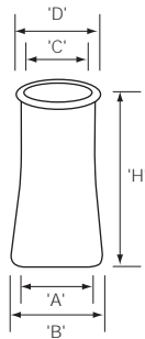
Square to Round Type 4D
