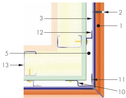
corner detail
